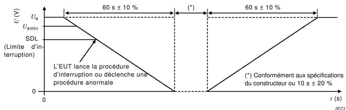
Figure 8 – Essai d'interruption/mise en route progressives
