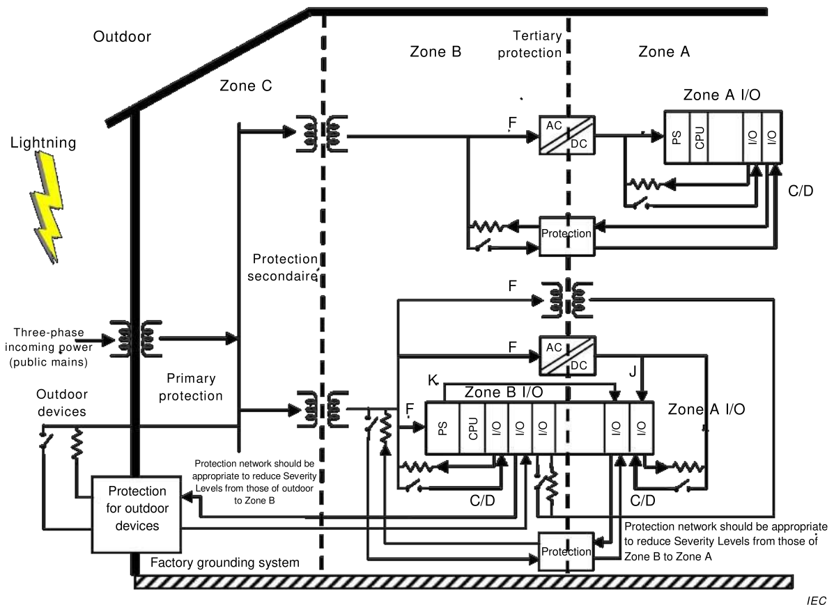
Figure 16 – EMC zones
